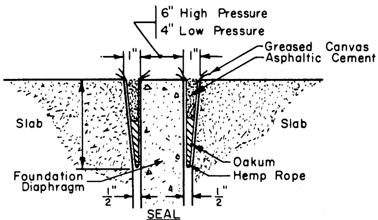
DETAIL C
